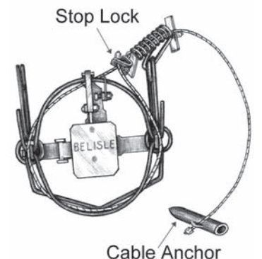
Spring-activated Cable Device
